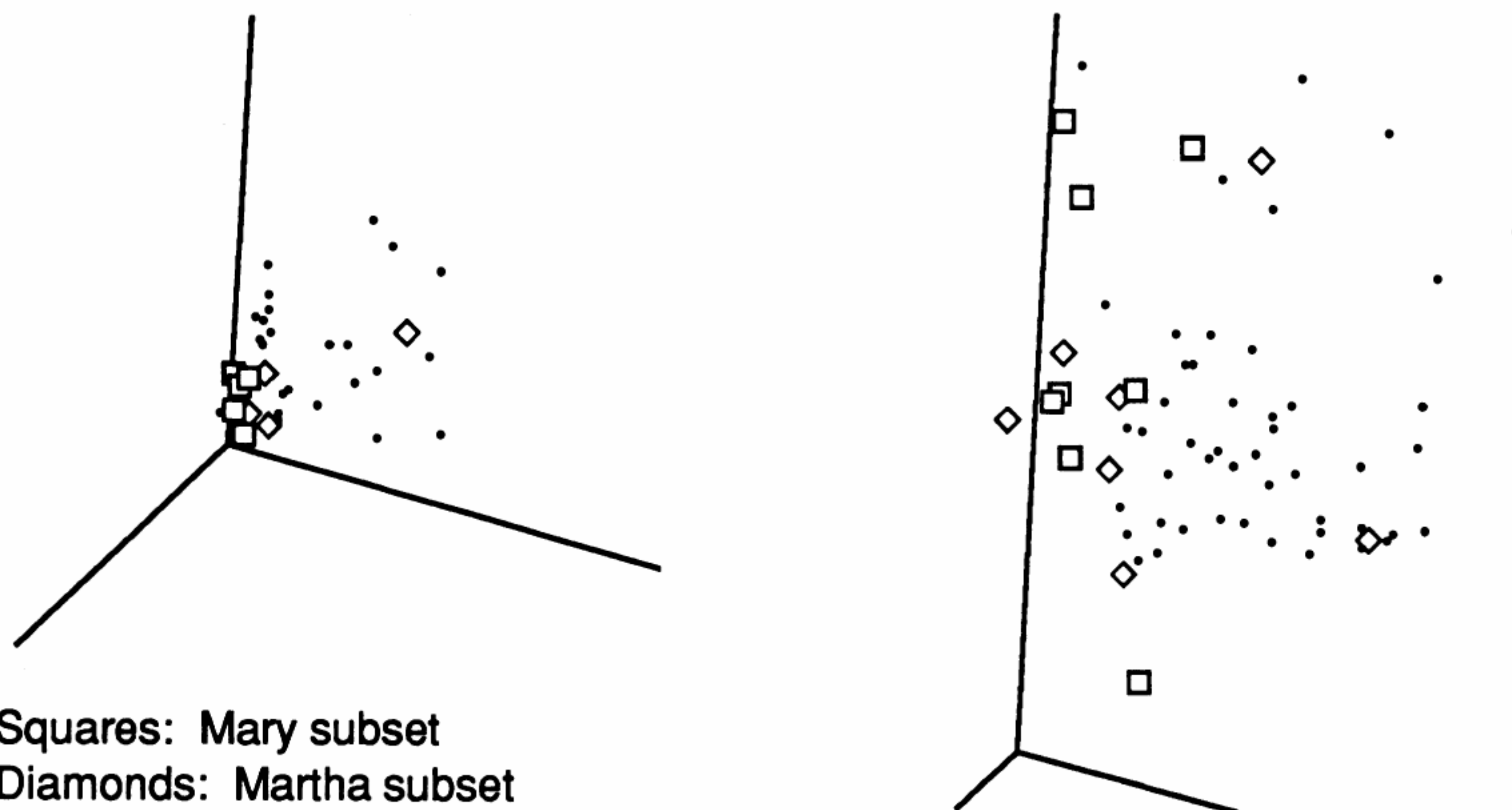
Fig. 7. Overlap of elements present in a statistical 'space' defined by axes representing the measured ratios to argon of iron, calcium, and potassium in the paper represented by several watermarks.
